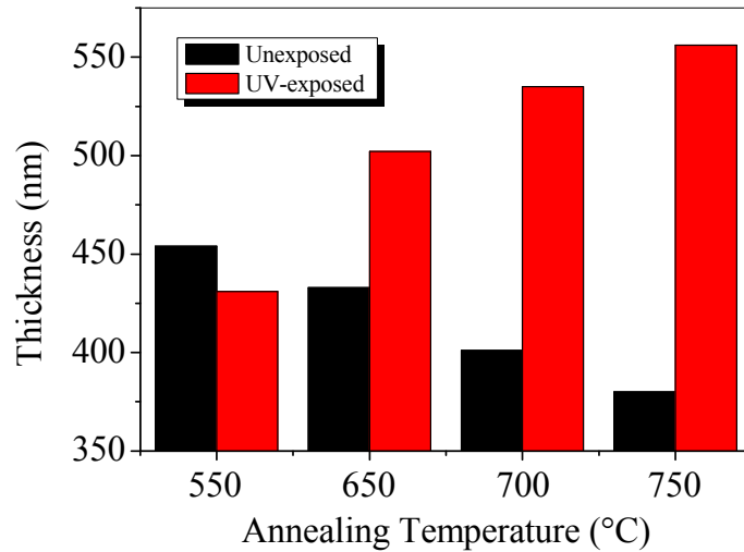
Figure 2.2.6: Thickness values of the films.
