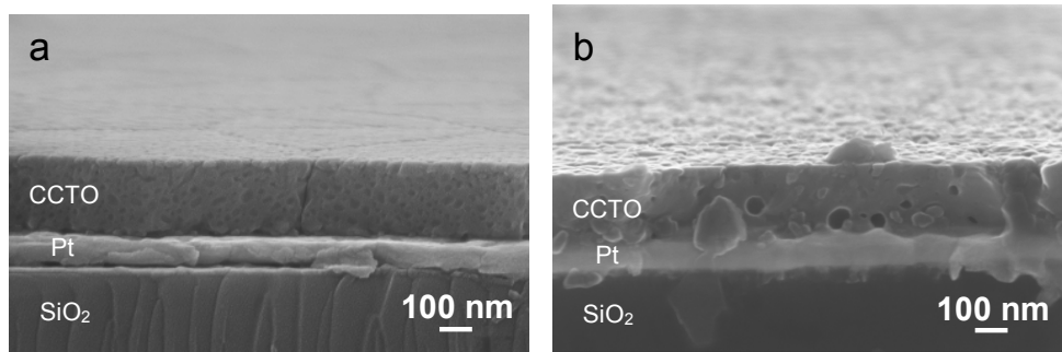
Figure 2.2.1: Cross-section FE-SEM micrographs of CCTO thin films: a) with (N13-07a) and b) without (N17-08) the NL, heated at 750^\circ\text{C} for 15 min.
