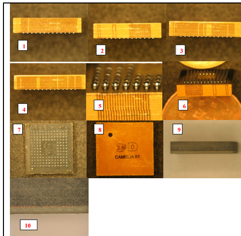
Figure 2.5.3: Detailed views of CAMELIA module : : side 1 view of module after laser patterning and varnishing (1) side 2 view of module after laser patterning and varnishing (2) side 3 view of module after laser patterning and varnishing (3) view as received from LETI ( 3), side 4 view of module after laser patterning and varnishing (4) tilted bottom view on BGA side showing solder balls (5) ) tilted bottom view on BGA side showing solder balls (6) BGA side after solder balling ( 7), top view after laser marking ( 8), side view after dicing and before metallization ( 9) same view showing copper tracks (10)
