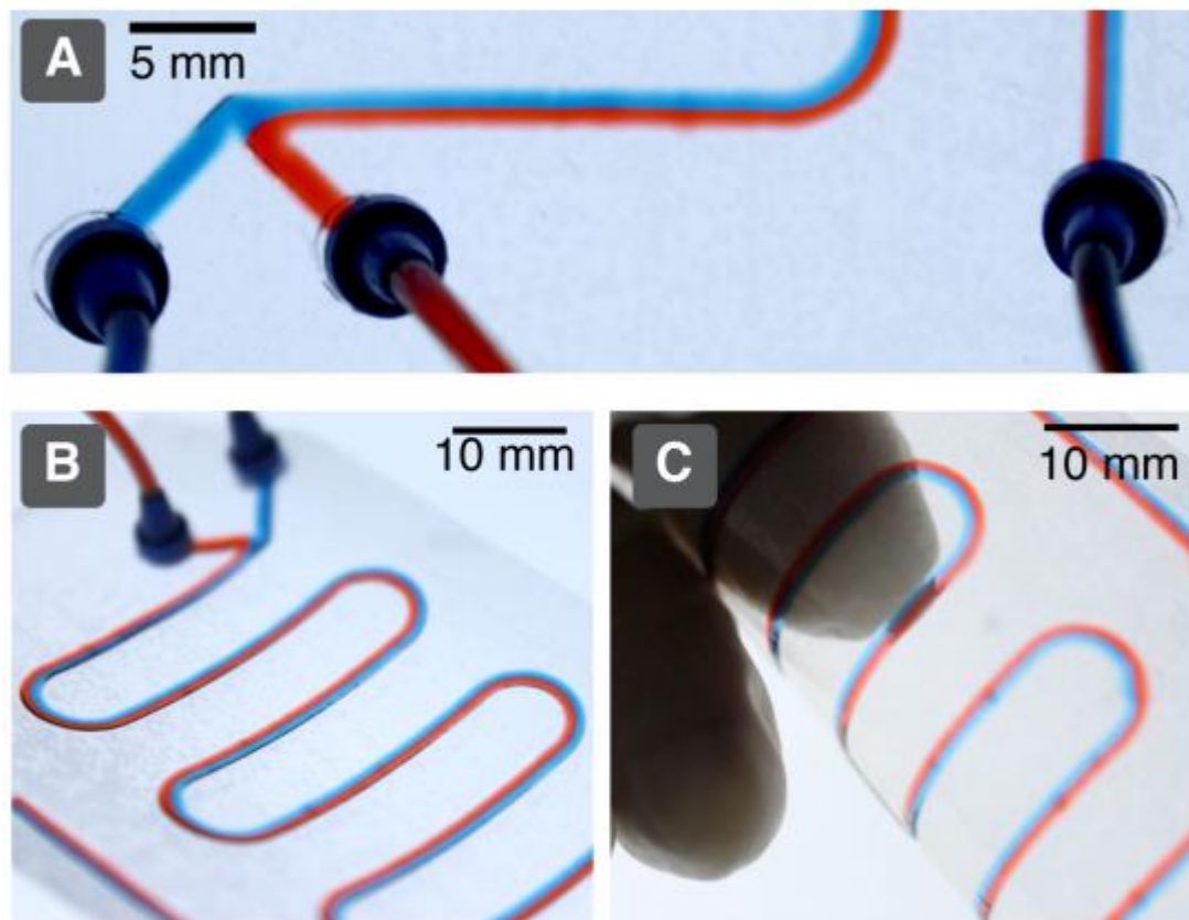
Figure 3. An all-cellophane microfluidic device. The red and blue colors are dyes in water, and flow at 100uL/min in laminar flow.
