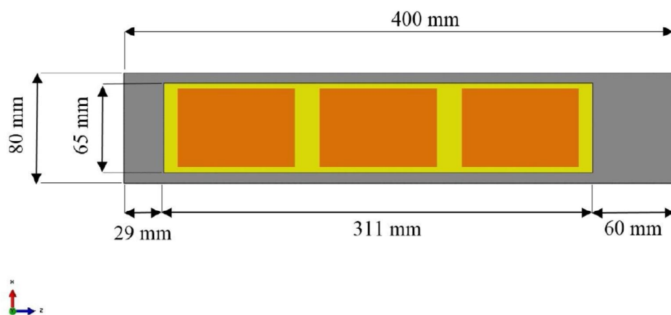
Layout and dimensions of a torsion specimen
