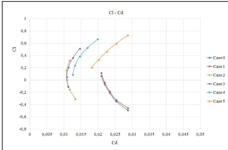
Drag polar curves for reference aileron-wing section ( h = 0 m, M = 0.17 ) – different aileron angles
