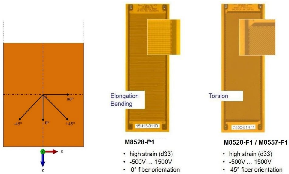
MFC types and fiber orientation
