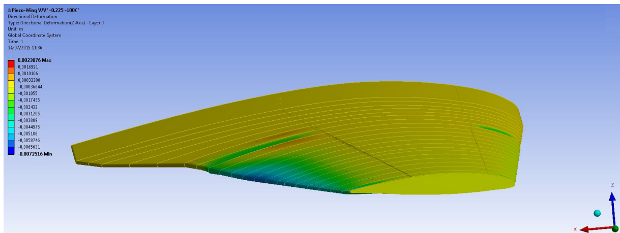
Deformed shape of the piezo-wing model (voltage + thermal pre-strain of the transition regions)
