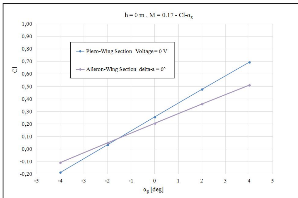
A comparison of Cl - \alpha_g curves for the examined wing sections ( h = 0 m, M = 0.17 )
