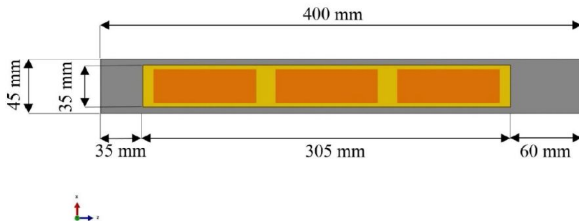
Layout and dimensions of a bending specimen
