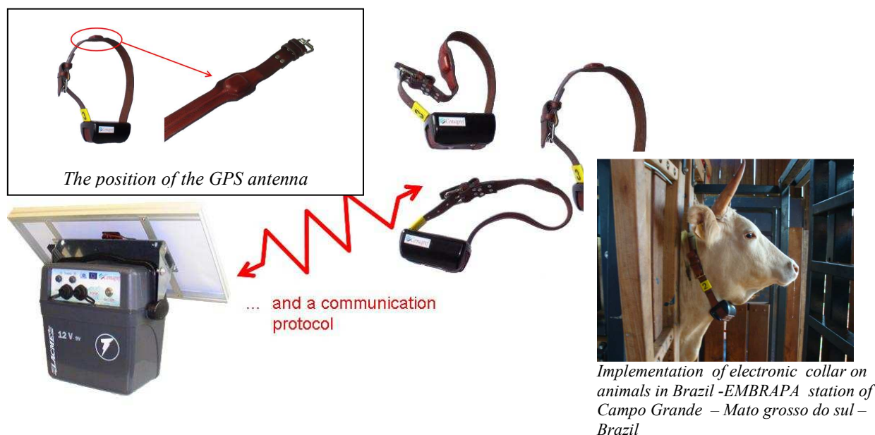
Figure on collar and base station system
