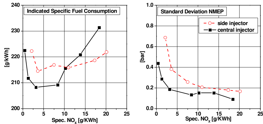
Fig. A2.2 Assessment of new lean burn combustion system Variation of relative Air/Fuel-Ratio, n = 2000 rpm, NMEP = 10 bar
