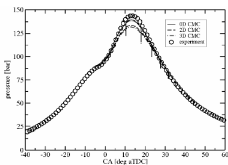
Fig. B1. 11: Measured and predicted pressure trace for a diesel engine. Experimental data and engine geometry from Y.M. Wright (PhD Thesis, 2005, ETH Zurich).
