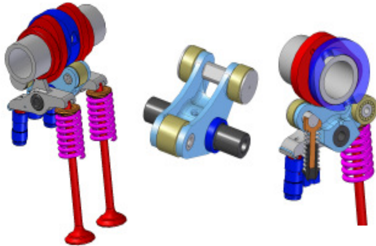
Figure A1.5 : Summing rocker system and concentric camshaft
