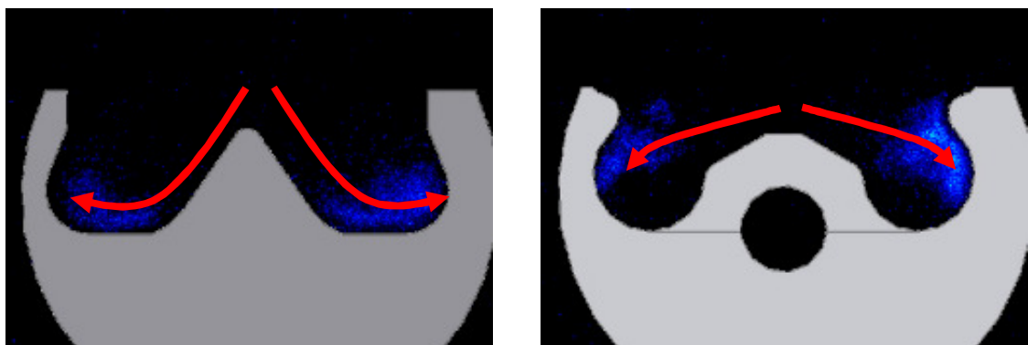
Figure A1.1: CH-radical images taken at 835 \mu s after the start of the electrical pulse for the 1200 bar and 264 cc/min case. Left – NADI chamber. Right - Classic chamber.
