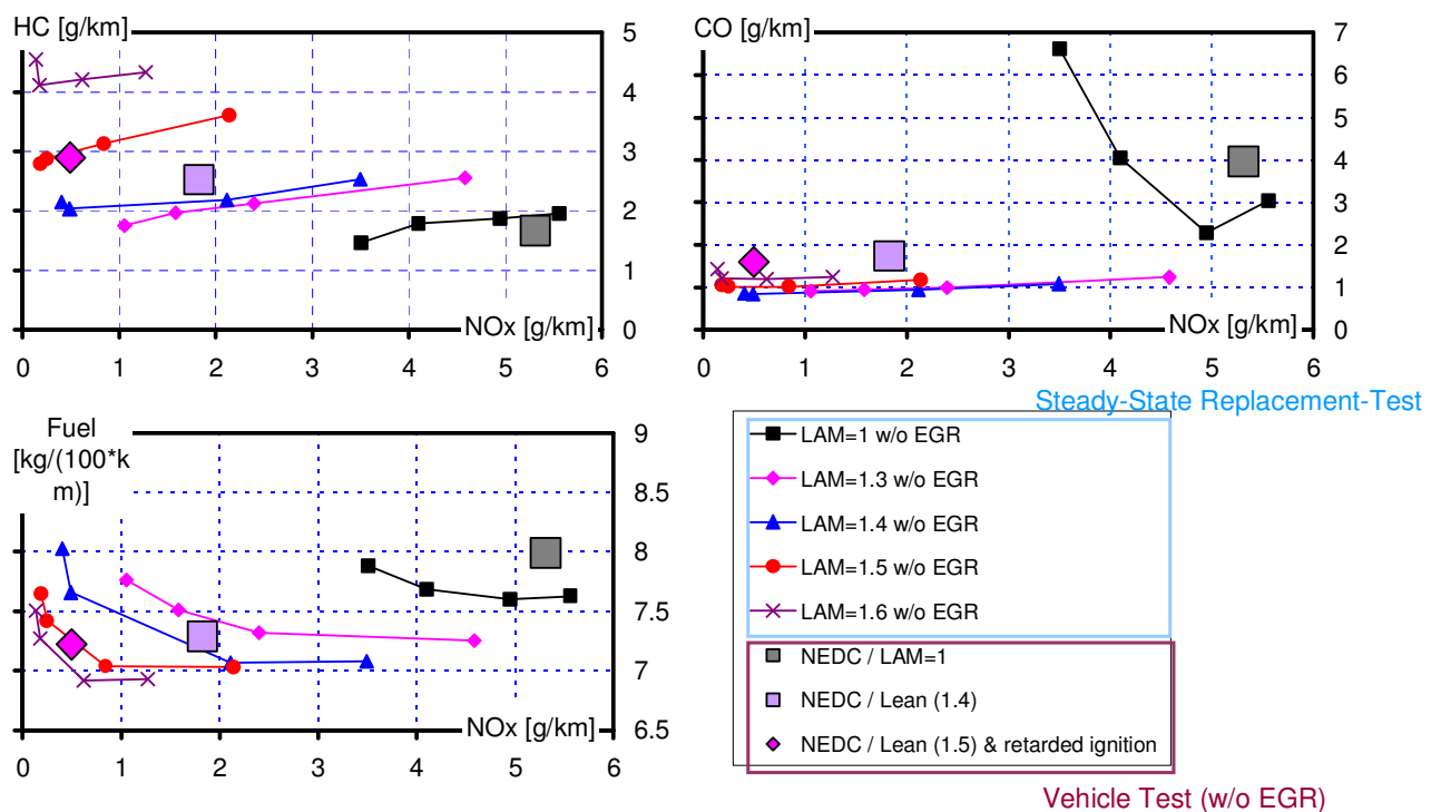
Fig. A3.18 Result comparison vehicle testing / Steady-state replacement-test
