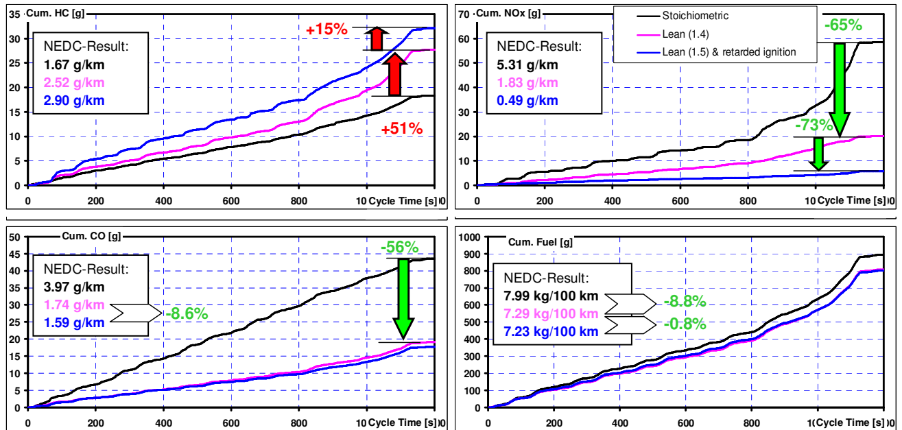
Fig. A3.17 NEDC testing (chassis dynamometer)
