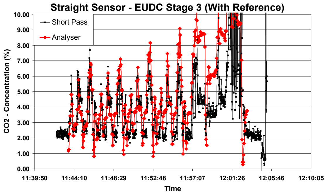
Figure 5.2.5. Evolution of CO 2 versus time as measured using the Mid IR optical fibre probe under standard engine test conditions for sensor mounted underneath the vehicle
