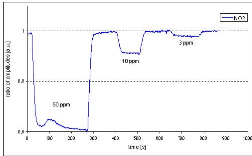
Figure 4.2.1.2. Transmission Of Different NO 2 Concentration Set By a Mixing Device, Recorded Using a Blue/UV LED And Photodiode.
