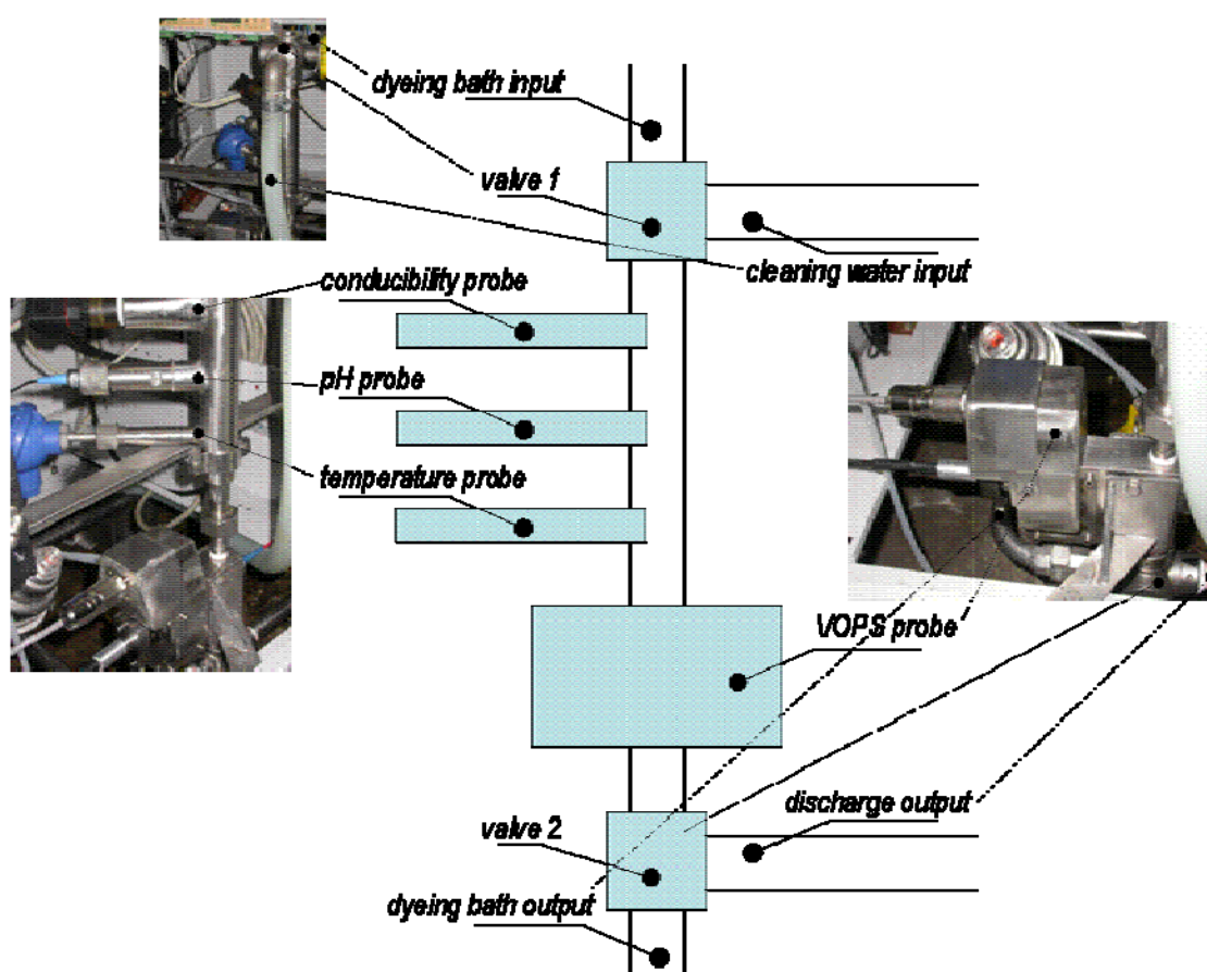
Figure 1 – Layout of EDY monitoring/control system
