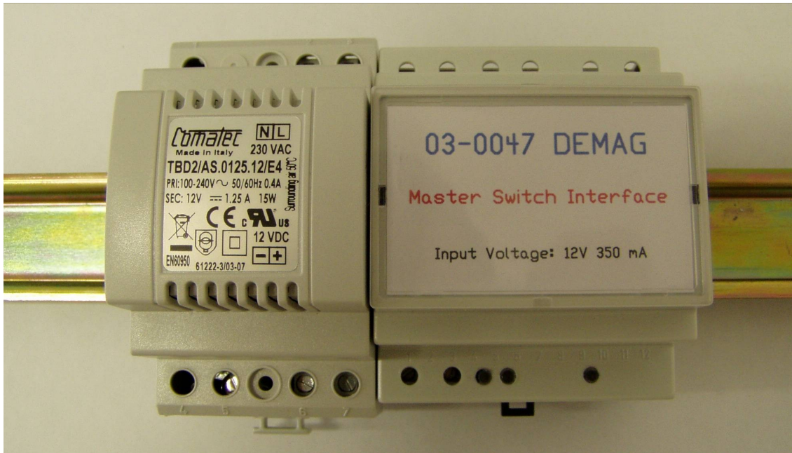
Figure 7: Overall view of the master switch unit (MSI + power supply)
