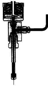
figure 2 Water jet cutting head, principle.
