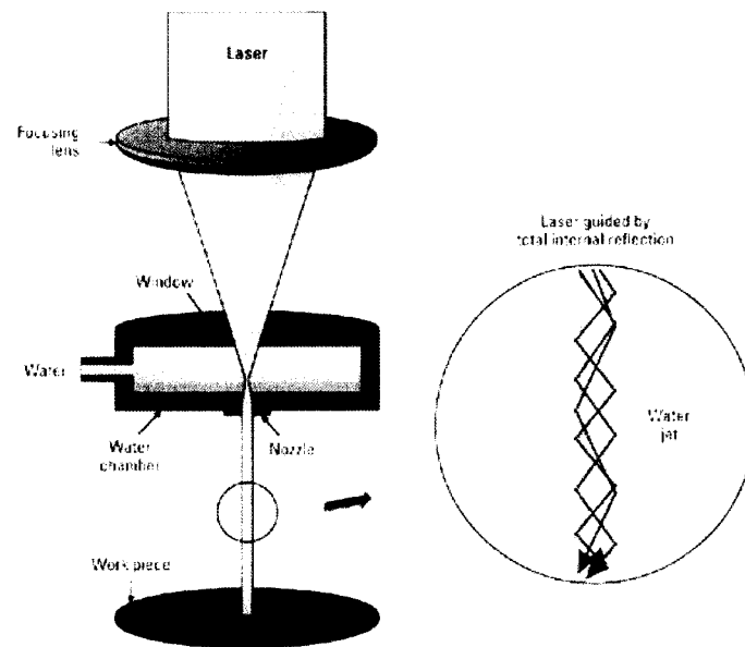
figure 7 Schematic overview of laser water jet principle.
