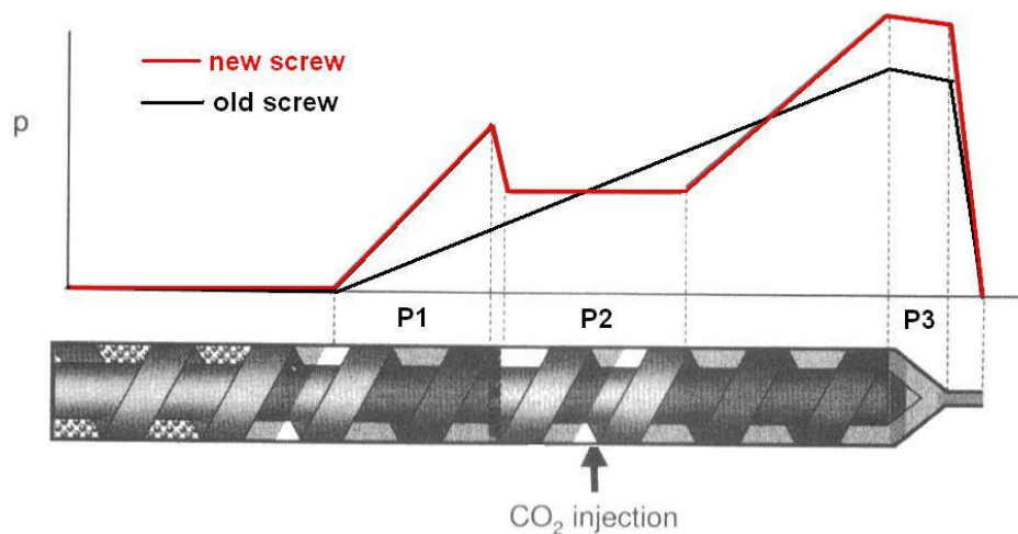
Figure 5: Comparison of pressure profiles between new and old screws
