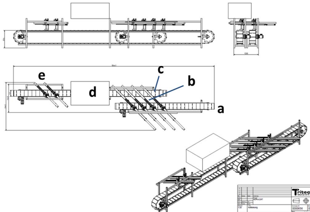
Figure 7: Drawing of the proposed set up for the demonstrator
