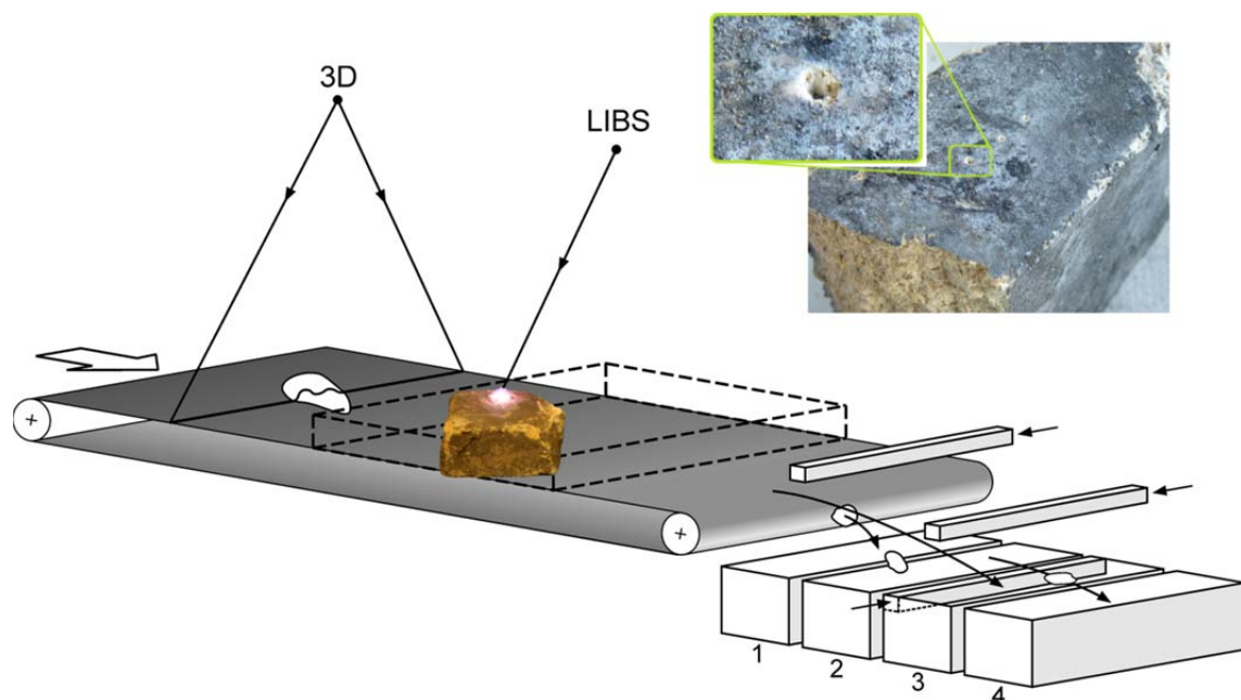
Figure 1: Basic principle of LIBS system in a sorting system (shown here with pneumatic separation). Inlay: photography of laser-penetration of surface contamination
