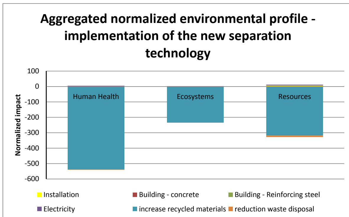
Figure 14: Aggregated normalized environmental profile of the implementation of the new separation technology, ReCiPe method (normalized against an average European in the year 2000)
