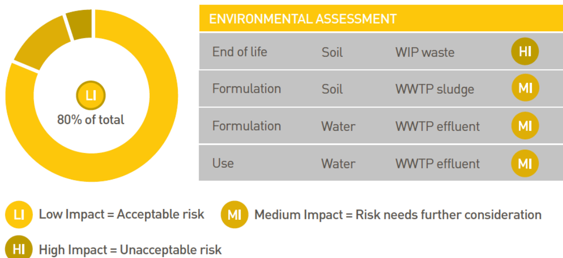
Example of the ecological risk portfolio along the lifecycle of a nanotechnology product.
