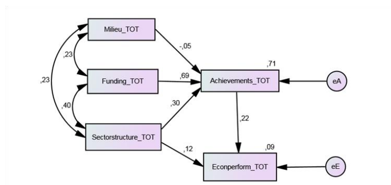
Figure 5 SEM model path and coefficients for total transport sector
