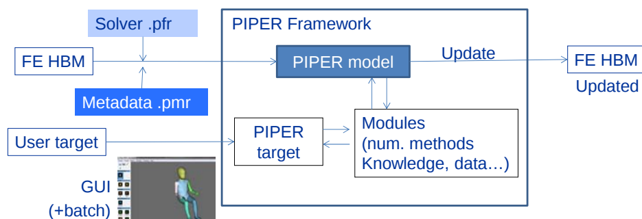
Figure 13: Overview of the PIPER framework and application. The use of external metadata and solver rule files prevents from putting any intellectual property from the FE HBM or the solver inside the framework, and enables HBM and solver neutrality. Modules can update the PIPER model (generated at import) and/or refine the target. New users can implement new modules and benefit from the overall developed infrastructure due to the independence of the framework from the solver of the HBM.
