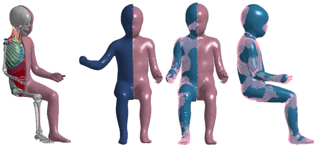
a) PIPER scalable child model b) Comparison with UMTRI shape (blue). Left: without postural adjustment. Right: with head and limbs from UMTRI shape aligned to the model skin.
