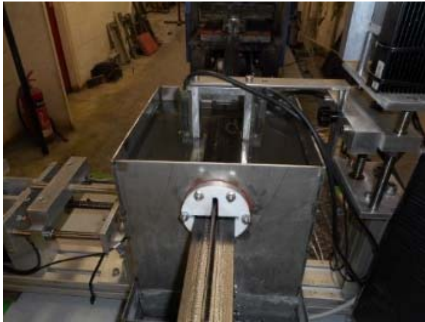
Figure 23. First profile exiting the water tank of the on-line QA system through the flange. Tight wipe ensures negligible water leakage and running on the surface.
