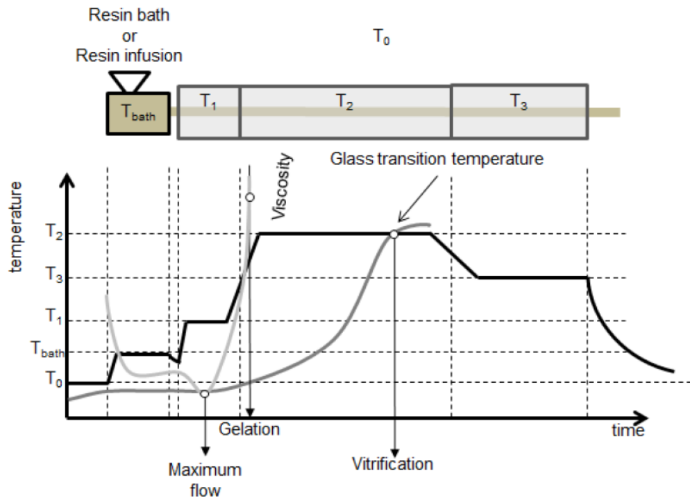
Figure 2. Cure design of stage 1. The temperature experienced by resin is plotted across a single die having two or more temperature regions
