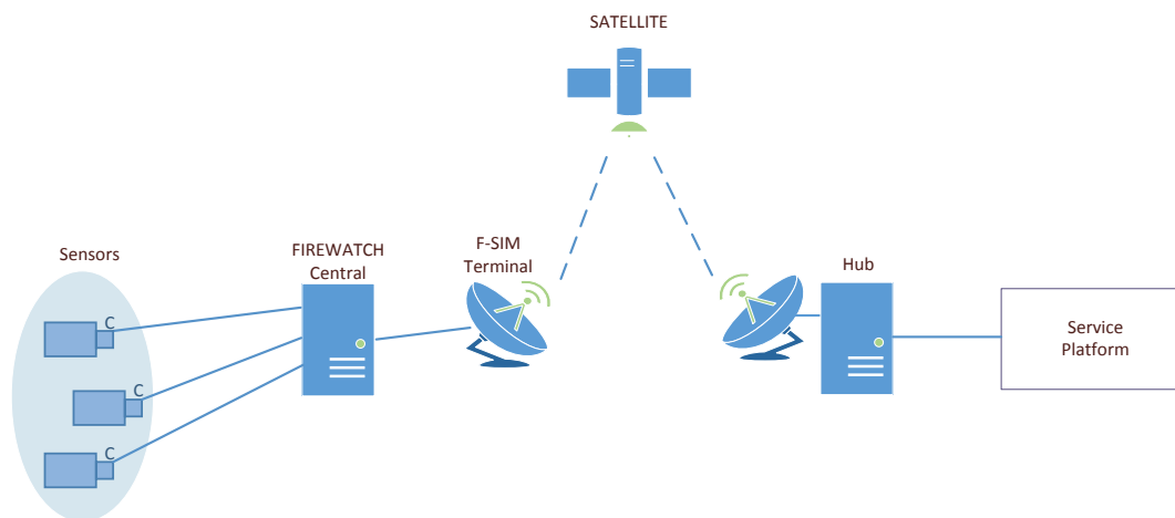
Figure 3-10: F-SIM Satellite System Integrated in PHAROS
