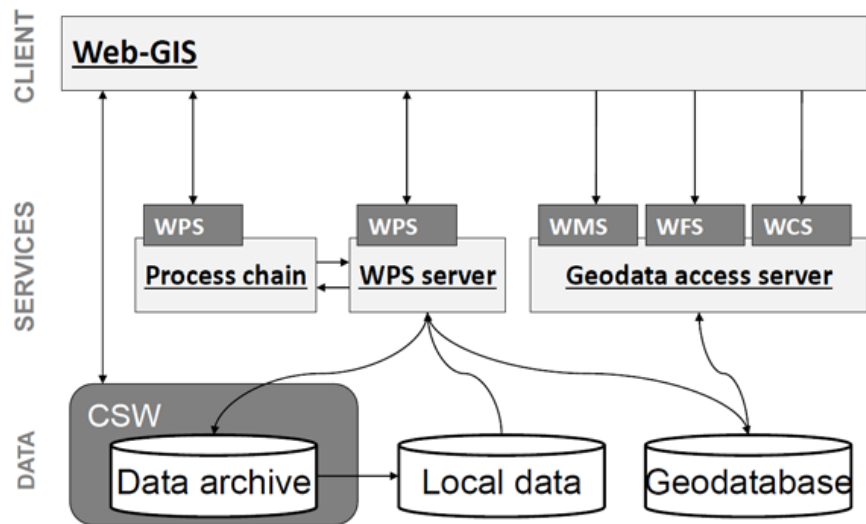
Figure 3-9: Implemented EO Services Technical Diagram
