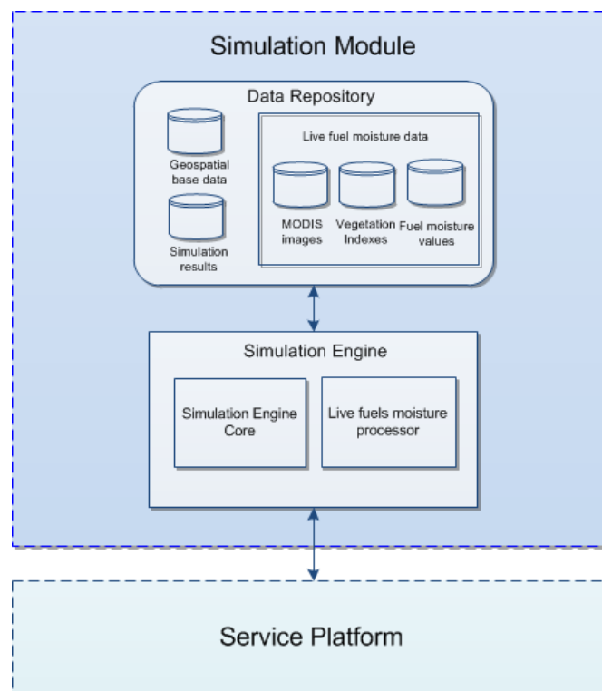
Figure 3-8: SM Overall Architecture
