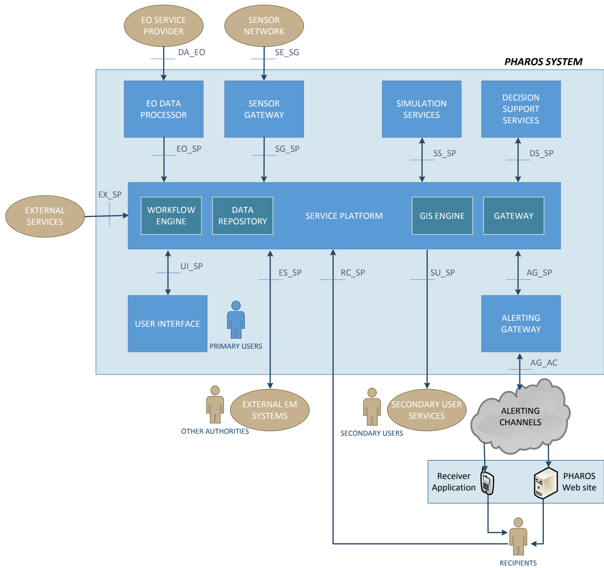
Figure 3-5: PHAROS Long Term Architecture
