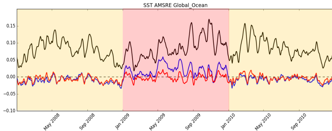
Figure 4. Global mean SST observation-minus-background (K) for the AMSRE microwave SST satellite from Jan 2008 to Dec 2010. Black line – no bias correction; blue line – bias correction using old scheme; red line – new bias scheme. In the middle year (2009), the reference satellite data from AATSR were withheld from all experiments.
