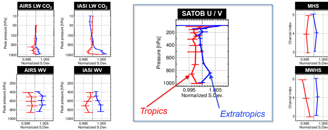
Figure 7. Differences in background standard deviation ( CERA - CNTR ) for selected satellites over the Tropics (red) and the extra-tropics (blue). Values below 1 (left of the vertical dashed line) indicate that the ocean coupling in the CERA system allows fitting better the observations. The comparison has been performed over September 2015-August 2016 and bars indicate the 95% confidence level.
