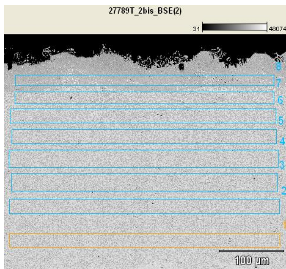
Figure 19:SEM micrograph of conical overaluminized
