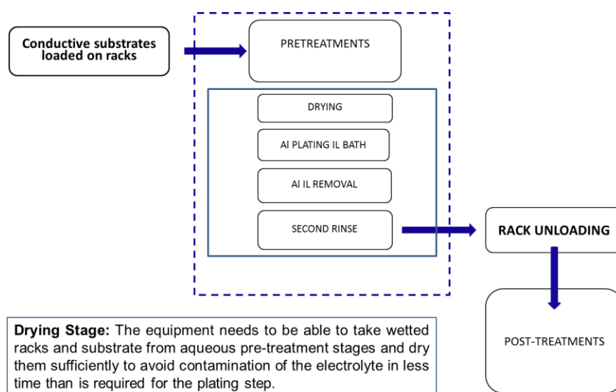
Figure 14: Diagram of the coating process
