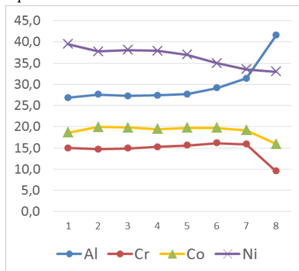
Figure 20:EDS profile of conical overaluminized
