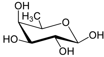
Figure 2: structure of L-fucose
