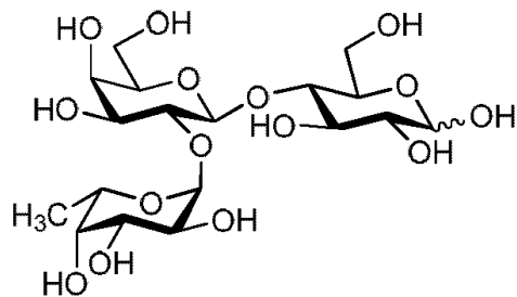
Figure 1: structure of 2'fucosyllactose
