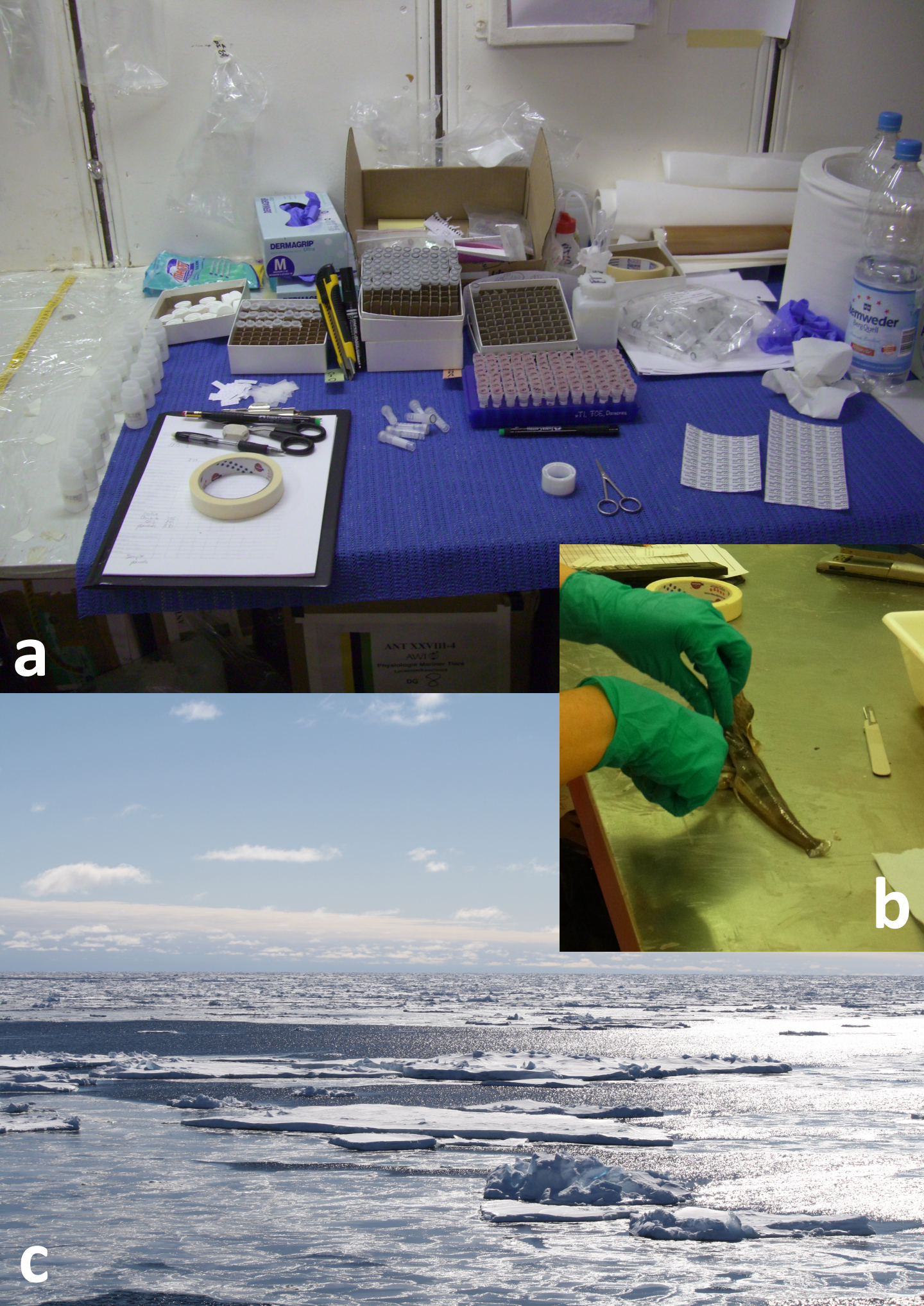
Figure 1. Antarctic notothenioid fish are endemic of Antarctic waters. To correctly apply conservation measures, we must investigate how they could react to the already observed global climate changes. (a) Lab-equipment ready for (b) sampling several tissues from notothenioid individuals for genetics during a polar cruise in Weddell Sea (Antarctica). (c) The sun is shining above the cold waters of the Weddell Sea. Photo credit Chiara Papetti
