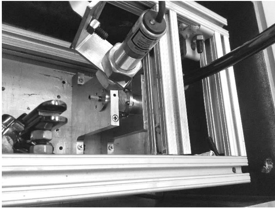
Figure 3 Spindle test rig with sensors
