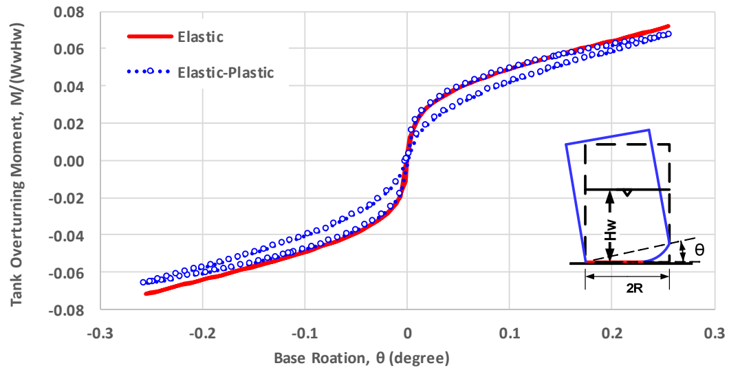
Fig. 17: Cyclic relationship between tank base rotation and overturning moment
