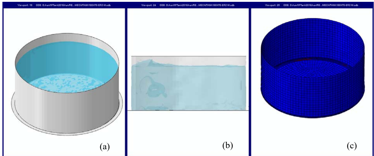
Fig. 20: CEL Modelling (a) before earthquake loading, (b) during loading and water sloshing, (c) tank during loading
